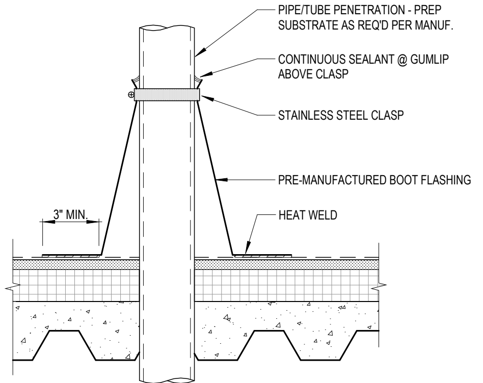
OAC - TYPICAL ROOF PENETRATION 13
