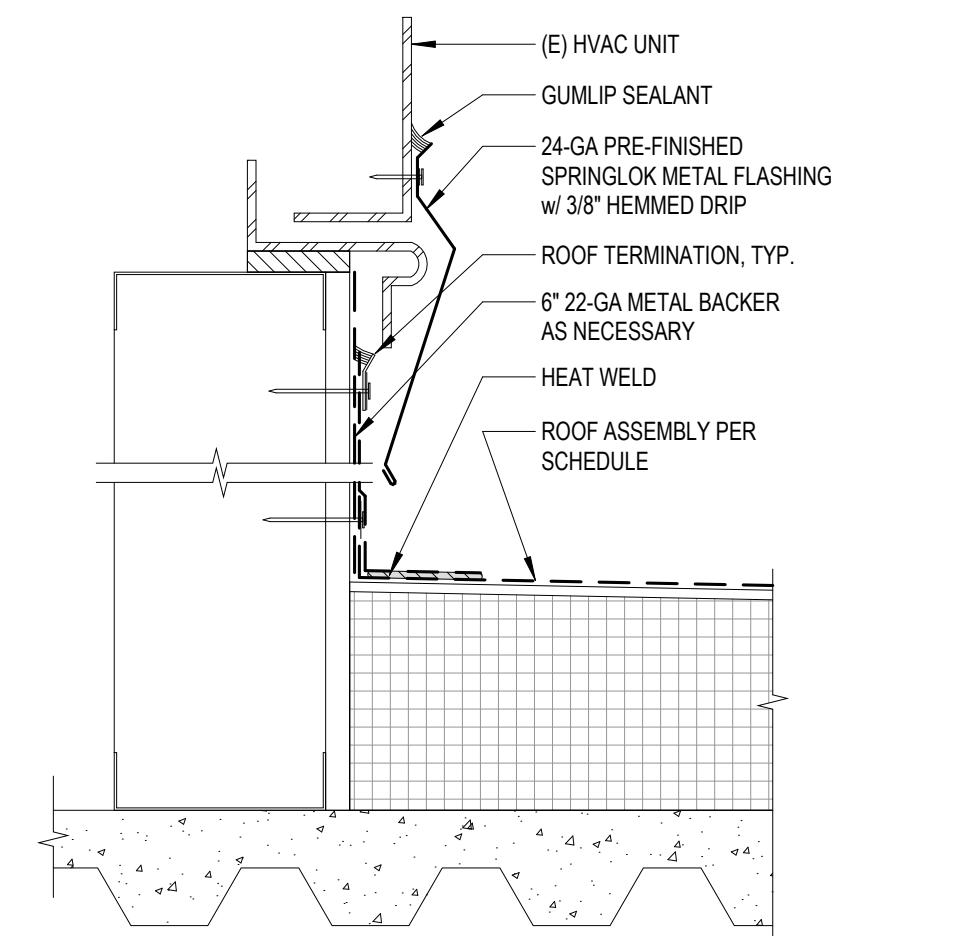
OAC - TYPICAL MECH CURB (UNIT STAYS IN PLACE) (12)
