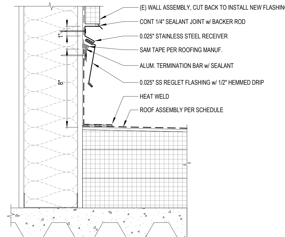
OAC - BASE OF WALL 6
