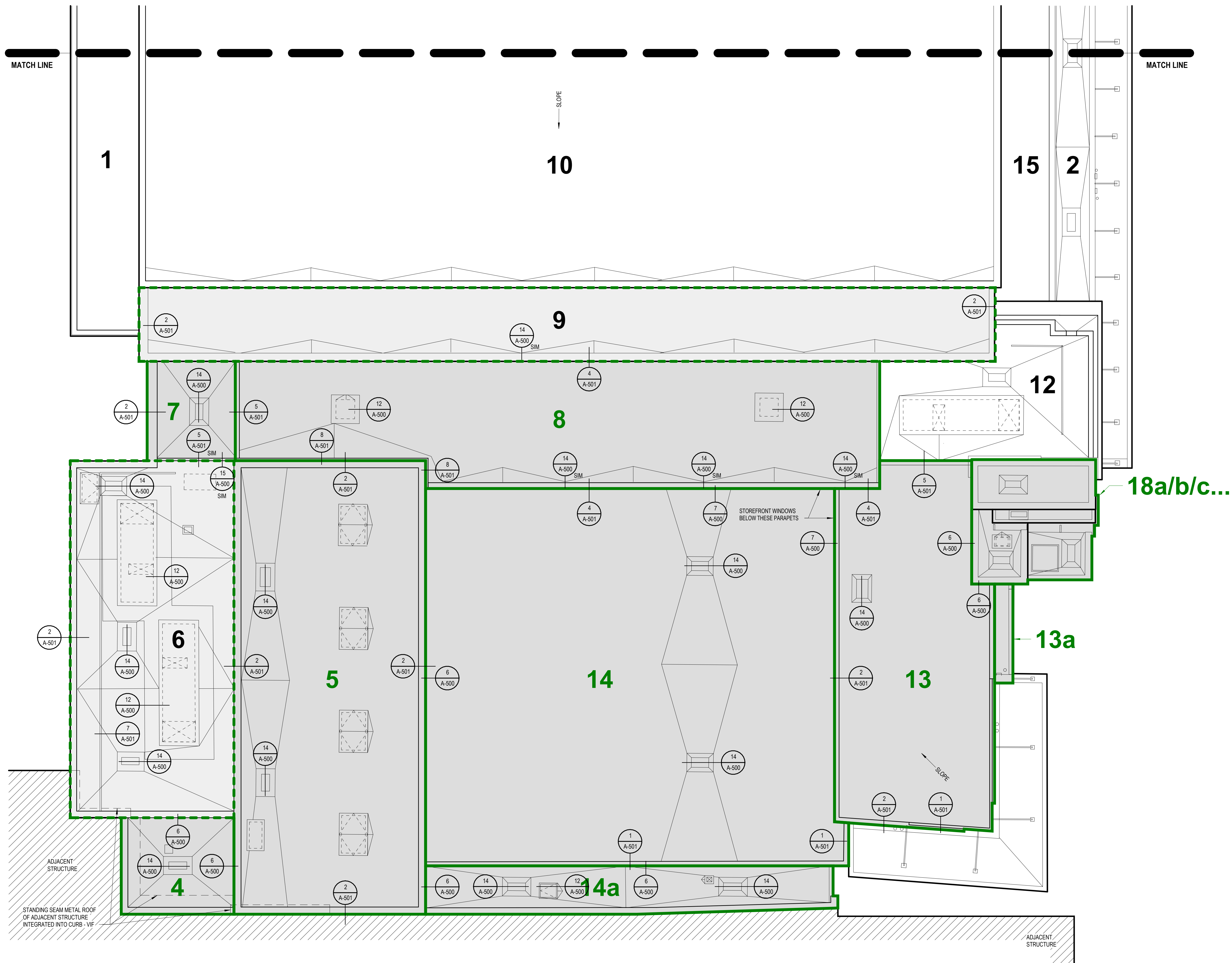
ROOF PLAN - WEST 1" = 10'-0"
