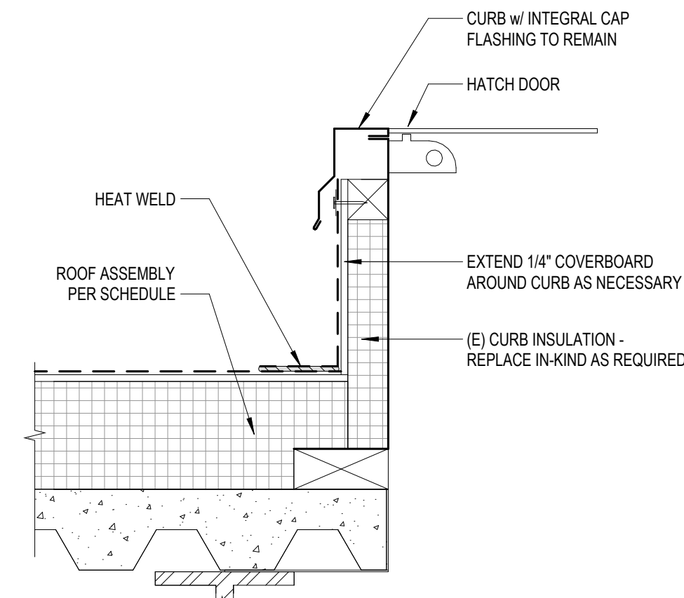
OAC - TYPICAL ROOF HATCH CURB 10
