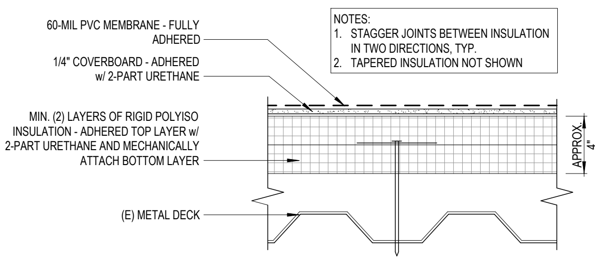
OAC - ROOF ASSEMBLY C 3
