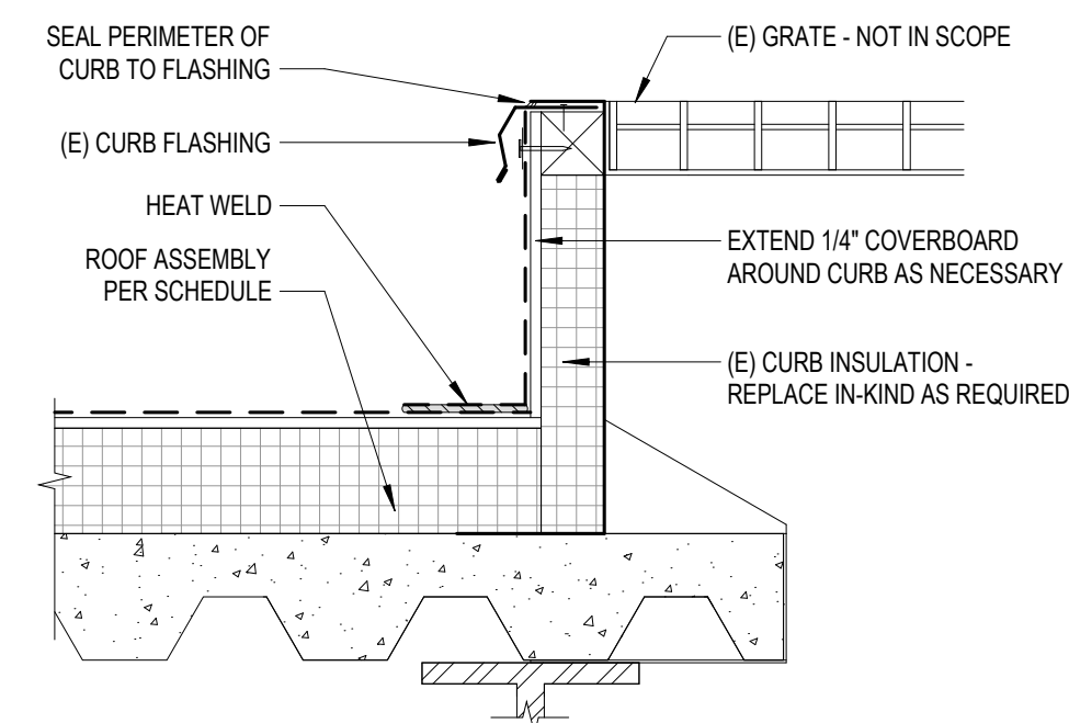
OAC - TYPICAL CURB AT GRATE 11
