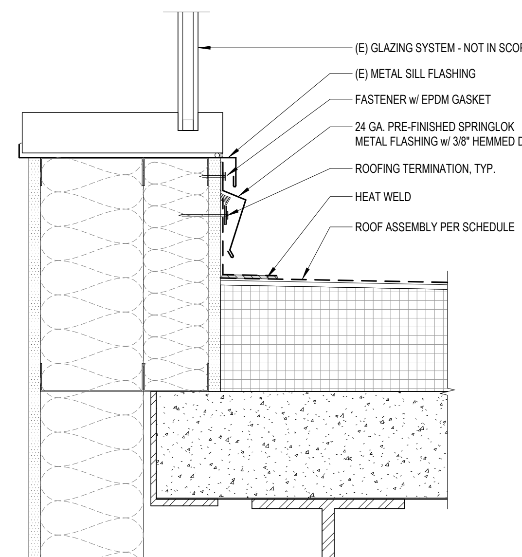
OAC - WINDOW SILL TO ROOF, TYP. (7)
