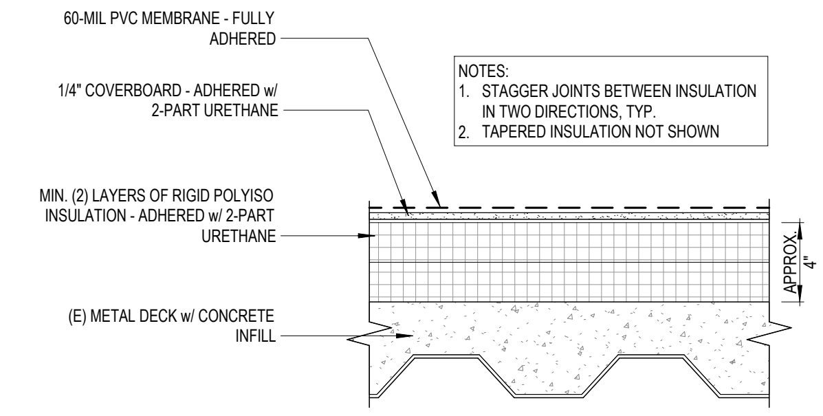
OAC - ROOF ASSEMBLY A 1
