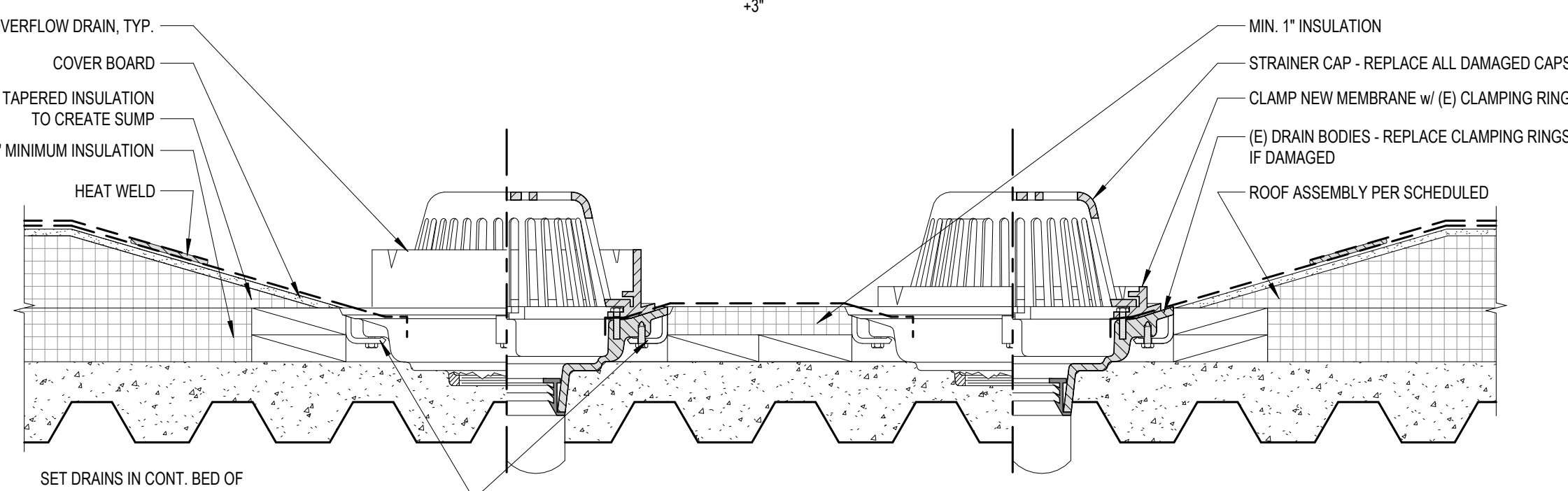
OAC - TYPICAL ROOF DRAIN w OVERFLOW 14
