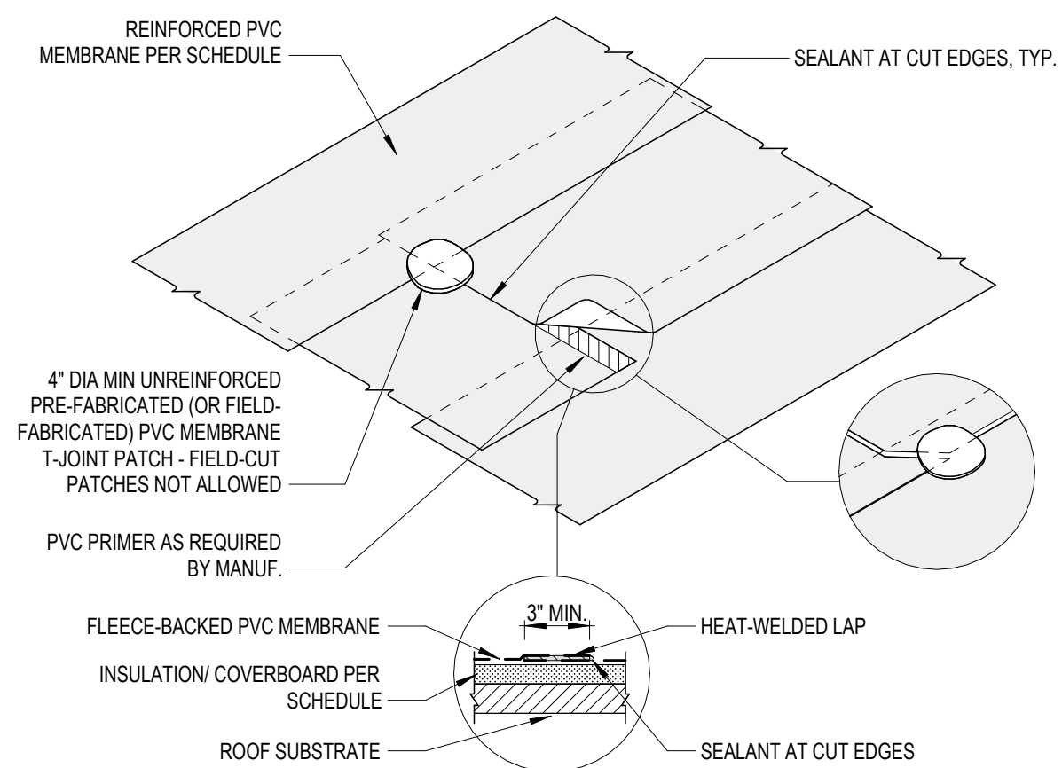
OAC - TYPICAL LAP & T-JOINT PATCH (4)
