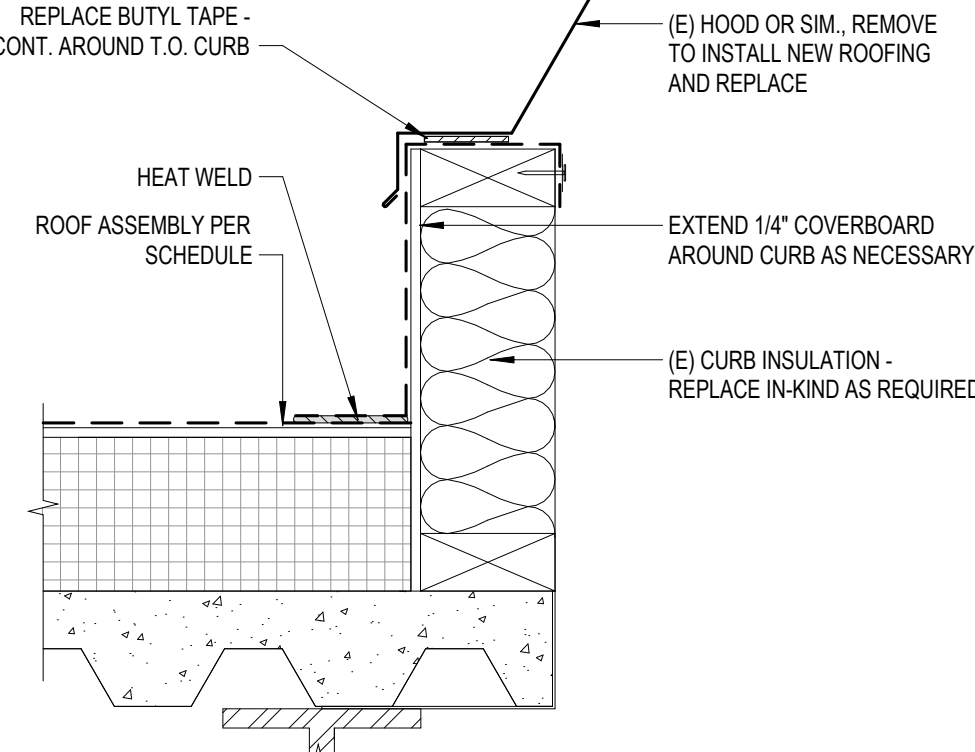
OAC - ROOF CURB 9
