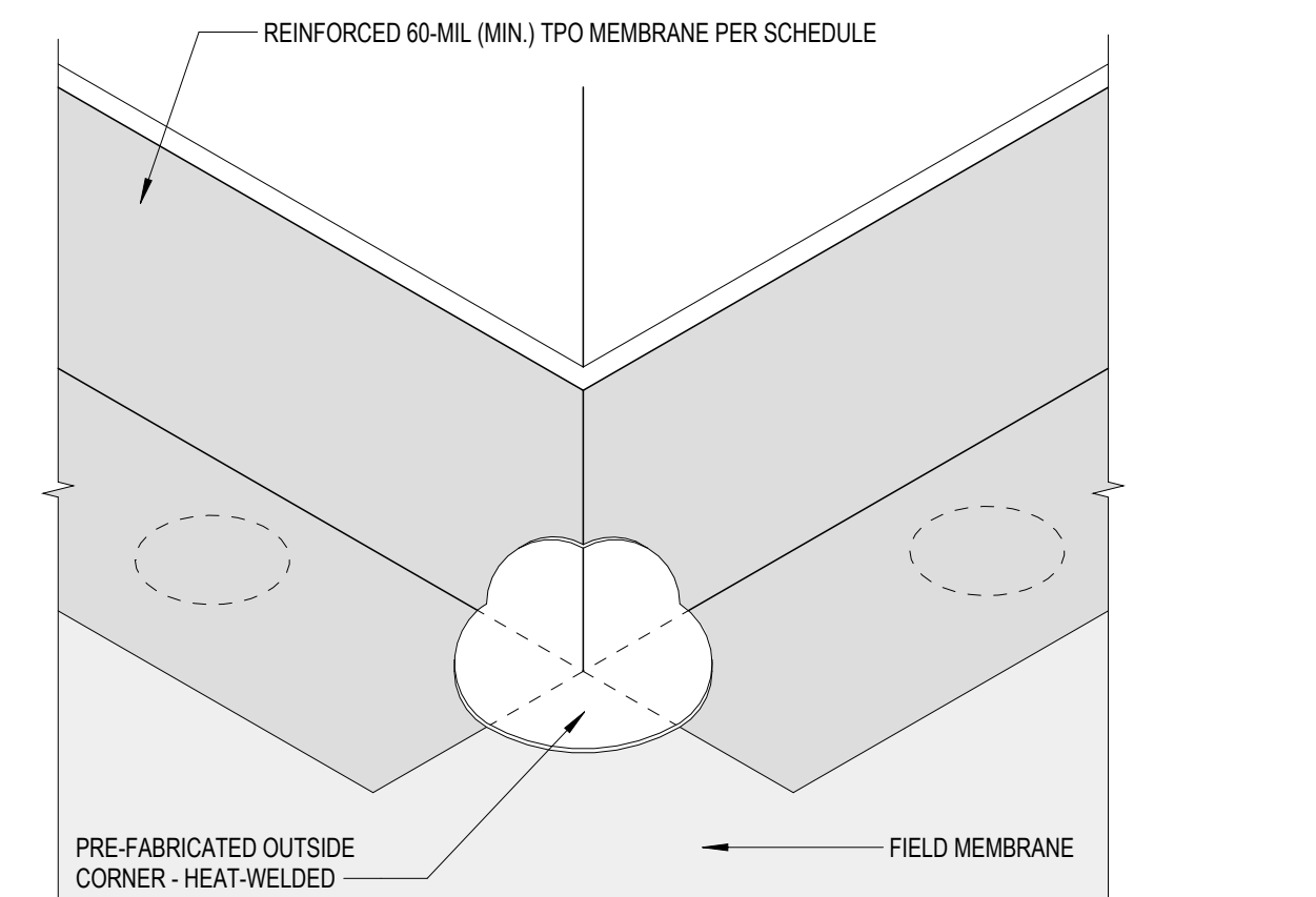
OAC - TYPICAL OUTSIDE CORNER 8
