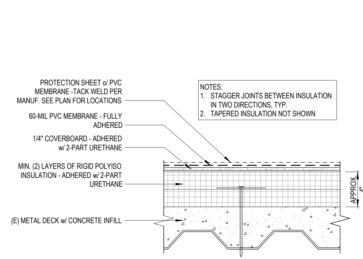
OAC - ROOF ASSEMBLY B (2)
