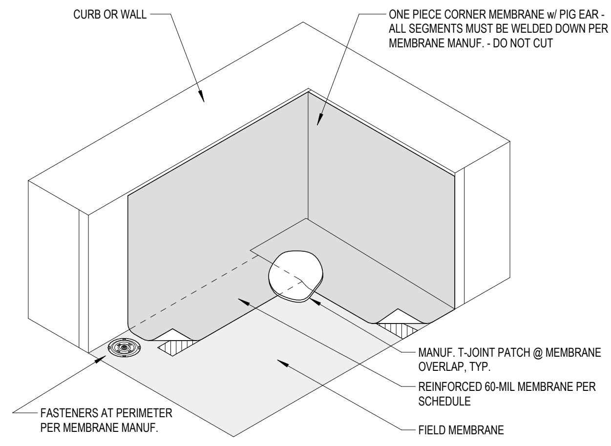
OAC - TYPICAL INSIDE CORNER 5
