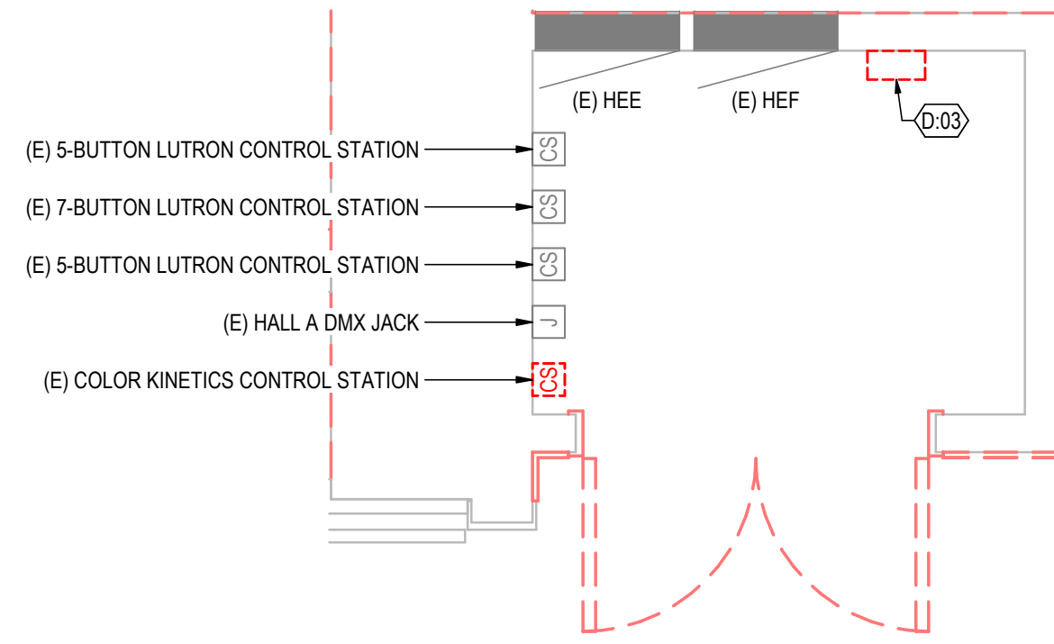
3 DEMO ENLARGED PLAN - ELEC 407B ED101 1/2" = 1'-0"
