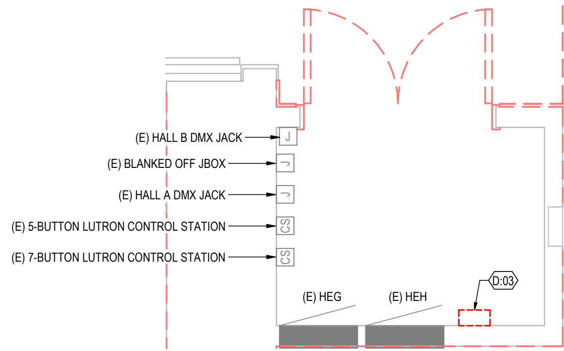
2 DEMO ENLARGED PLAN - ELEC 407A ED101 1/2" = 1'-0"
