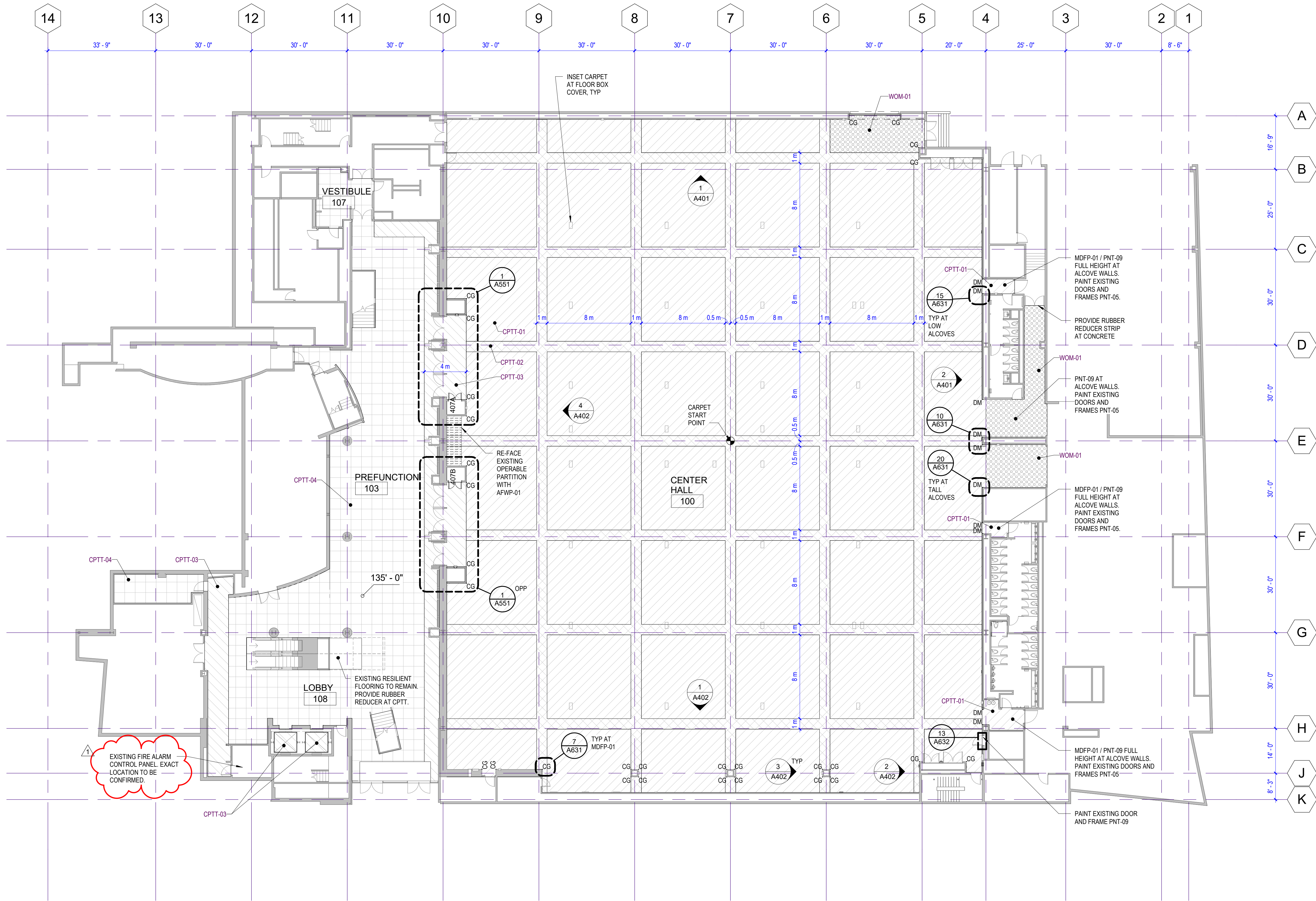
1 OVERALL PLAN - LEVEL 1 A101 1/16" = 1'-0"
