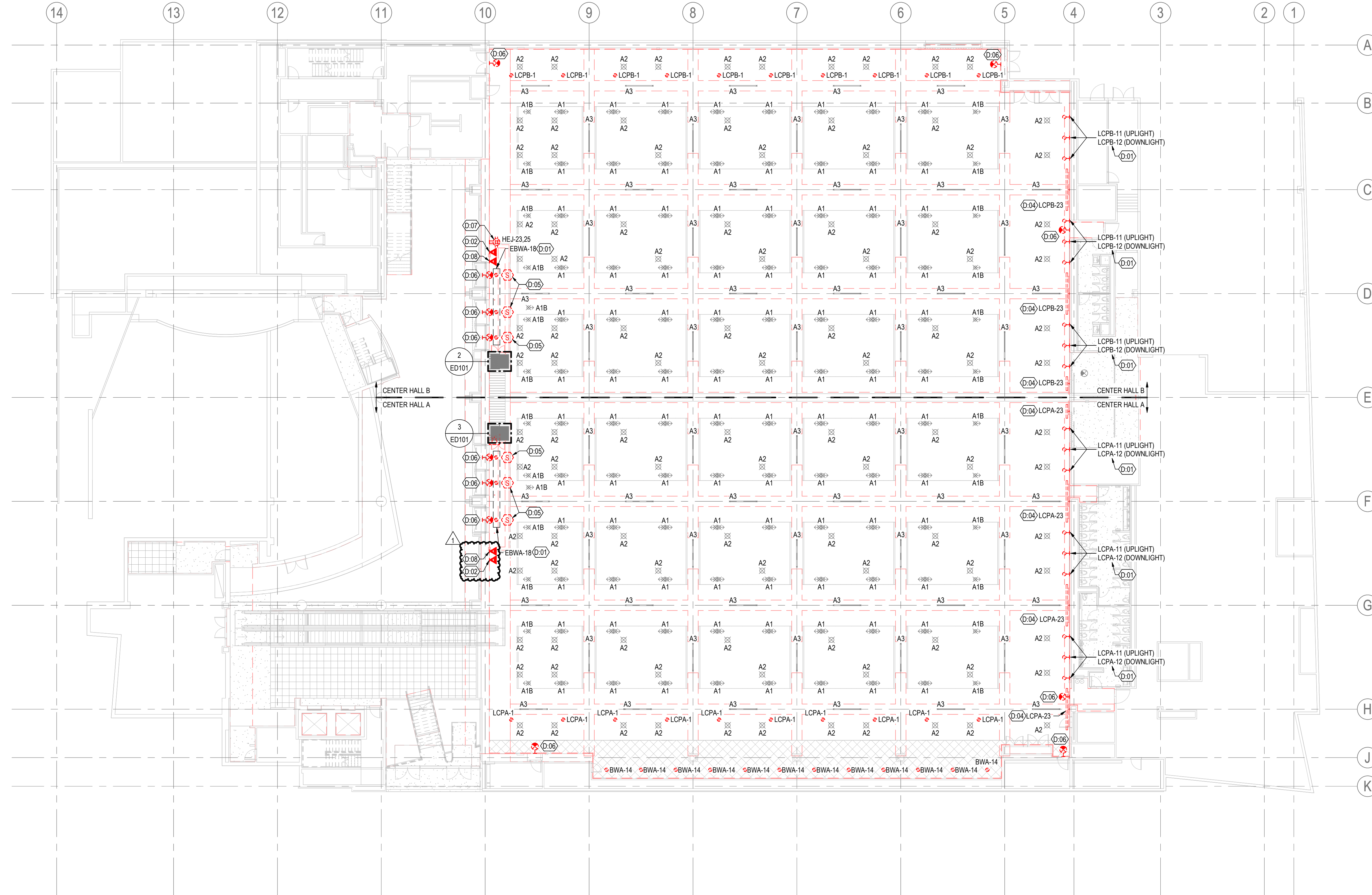
1 DEMO ELECTRICAL PLAN - LEVEL 1 ED101 1/16" = 1'-0"
